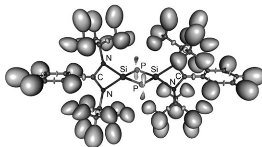
Figure 3. Representation of the ELI-d of compound 4 (isosurface value, \eta = 1.8 ).
